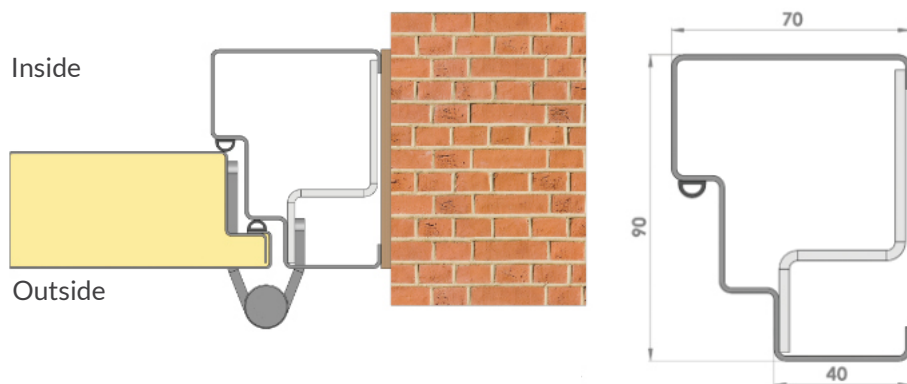
MITRED FRAME, OPEN TO OUTSIDE (LO)
