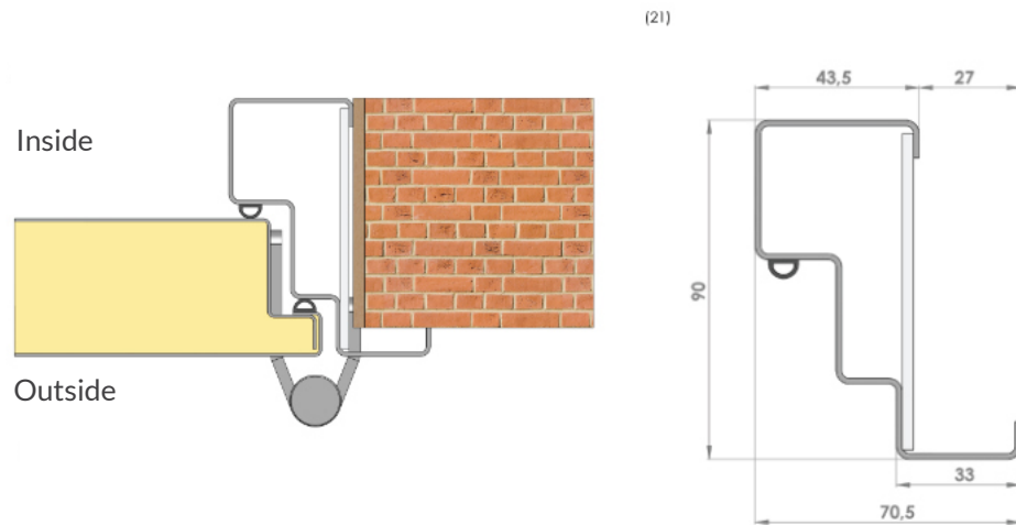
MITRED FRAME WITH MOULDINGS, OPEN TO OUTSIDE (MO)
