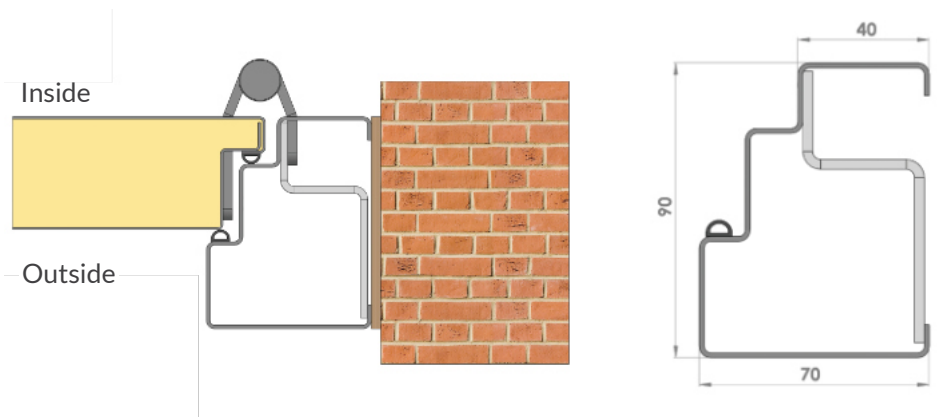
MITRED FRAME, OPEN TO INSIDE (LI)
